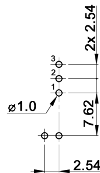
P.C. MOUNTING
