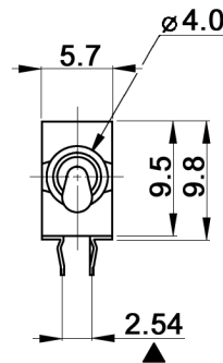
P.C. MOUNTING
