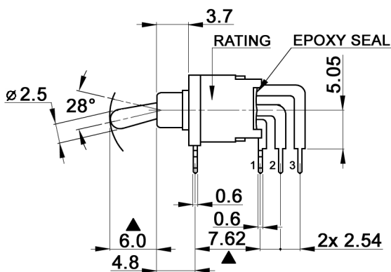
toggle shown in pos. a
